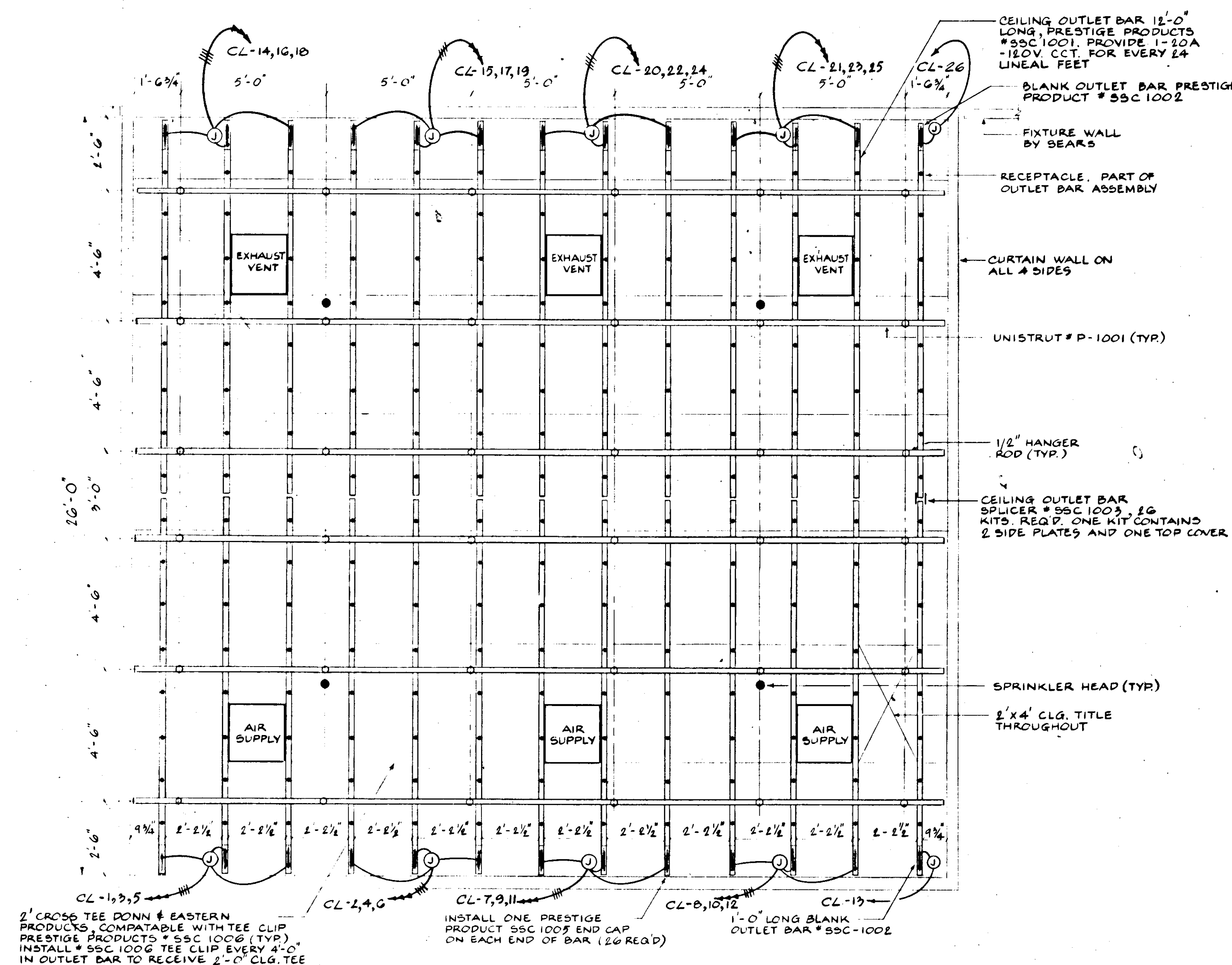
PLAN VIEW SCALE: 3/8" = 1'-0"
