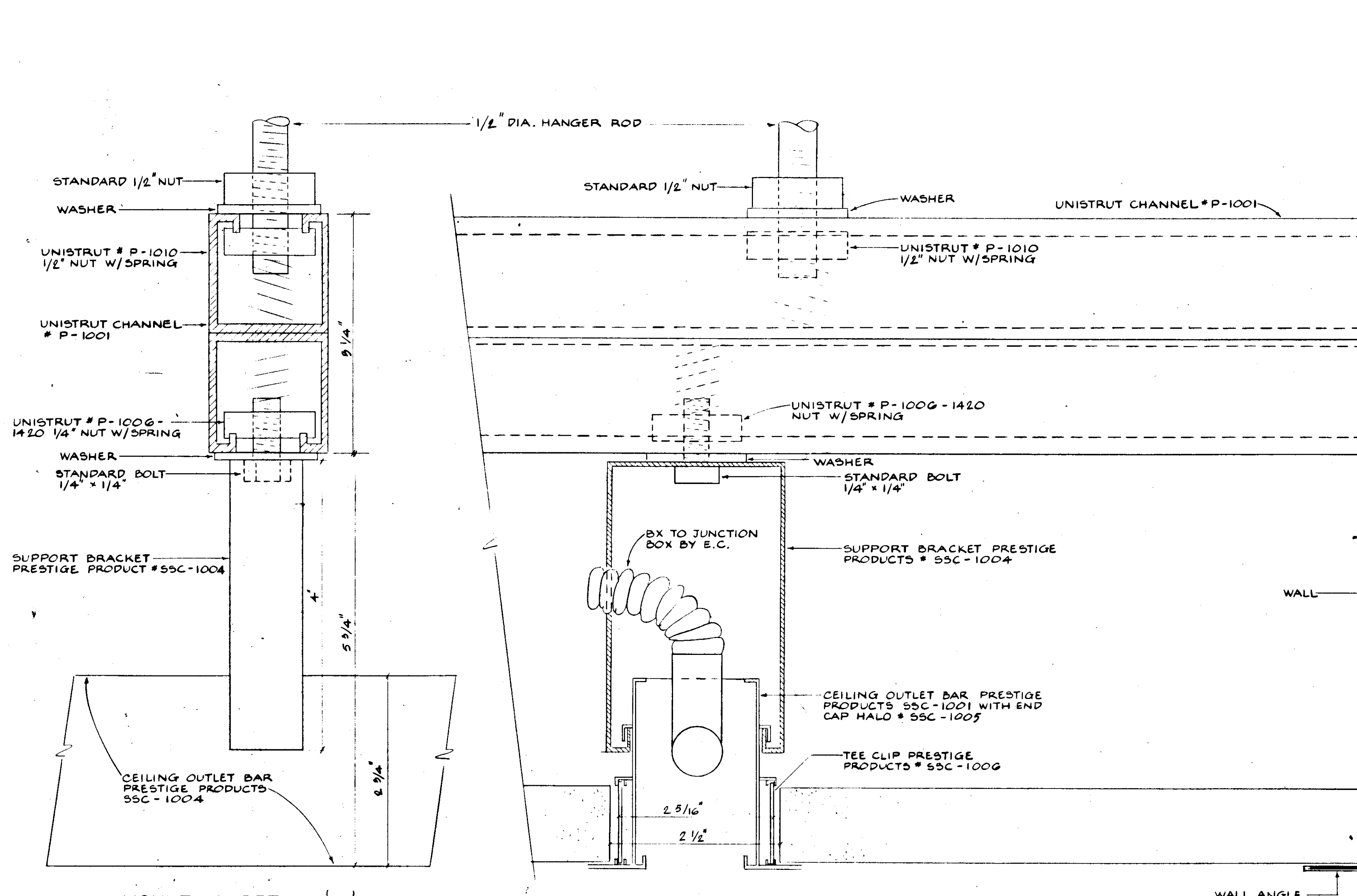
MOUNTING DETAIL 'B' FULL SCALE
