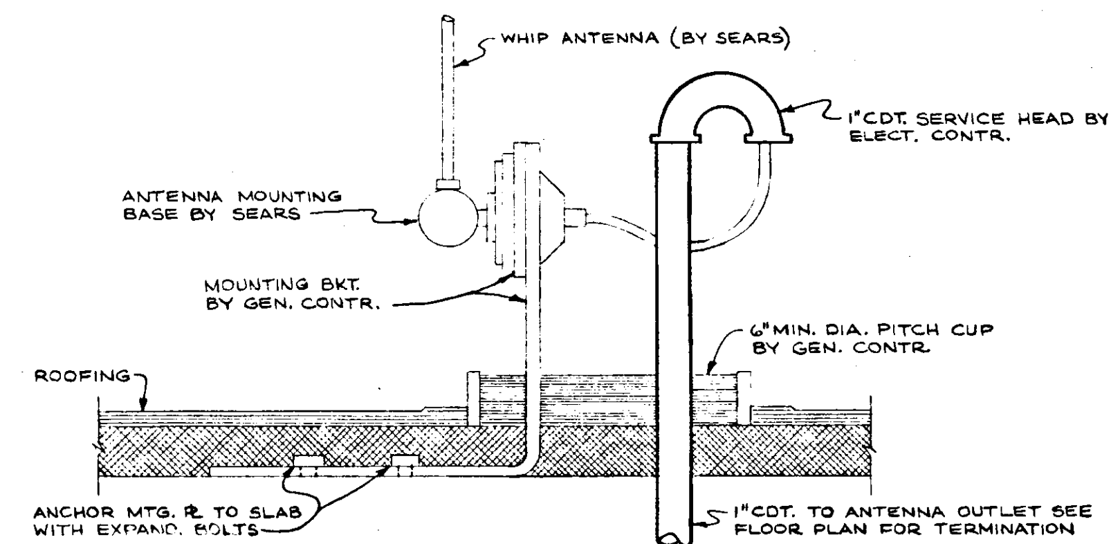
AUTO. CENTER RADIO ANTENNA DETAIL
