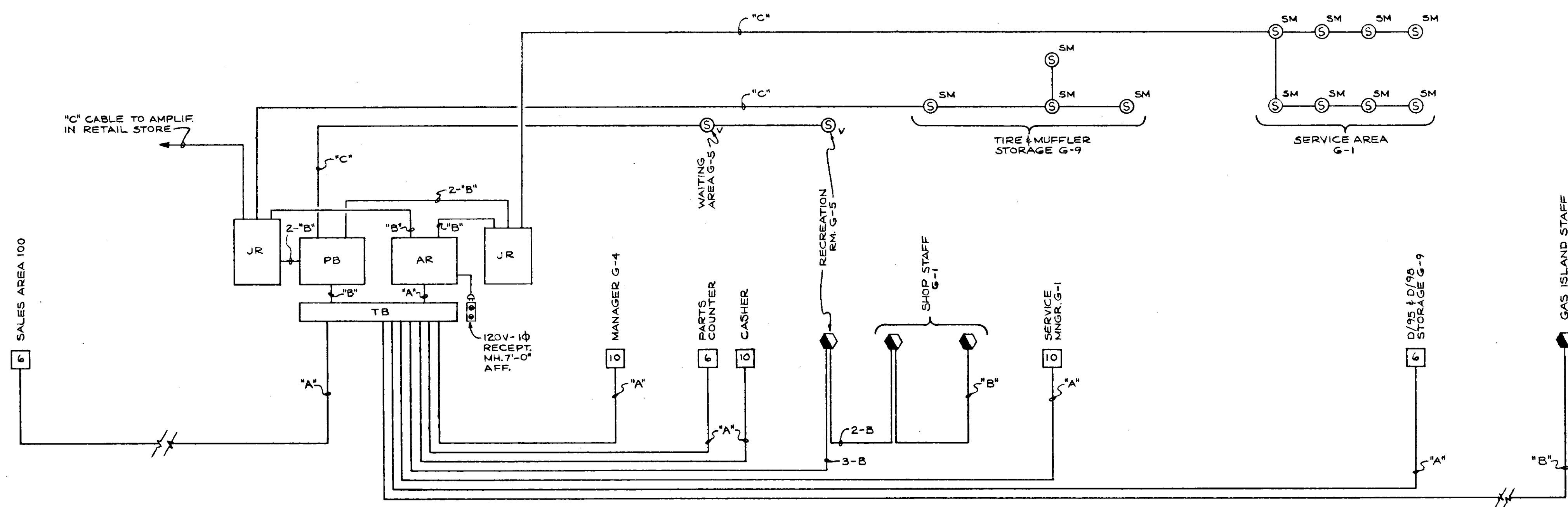
AUTO CENTER INTERCOM SYSTEM RISER DIAGRAM
