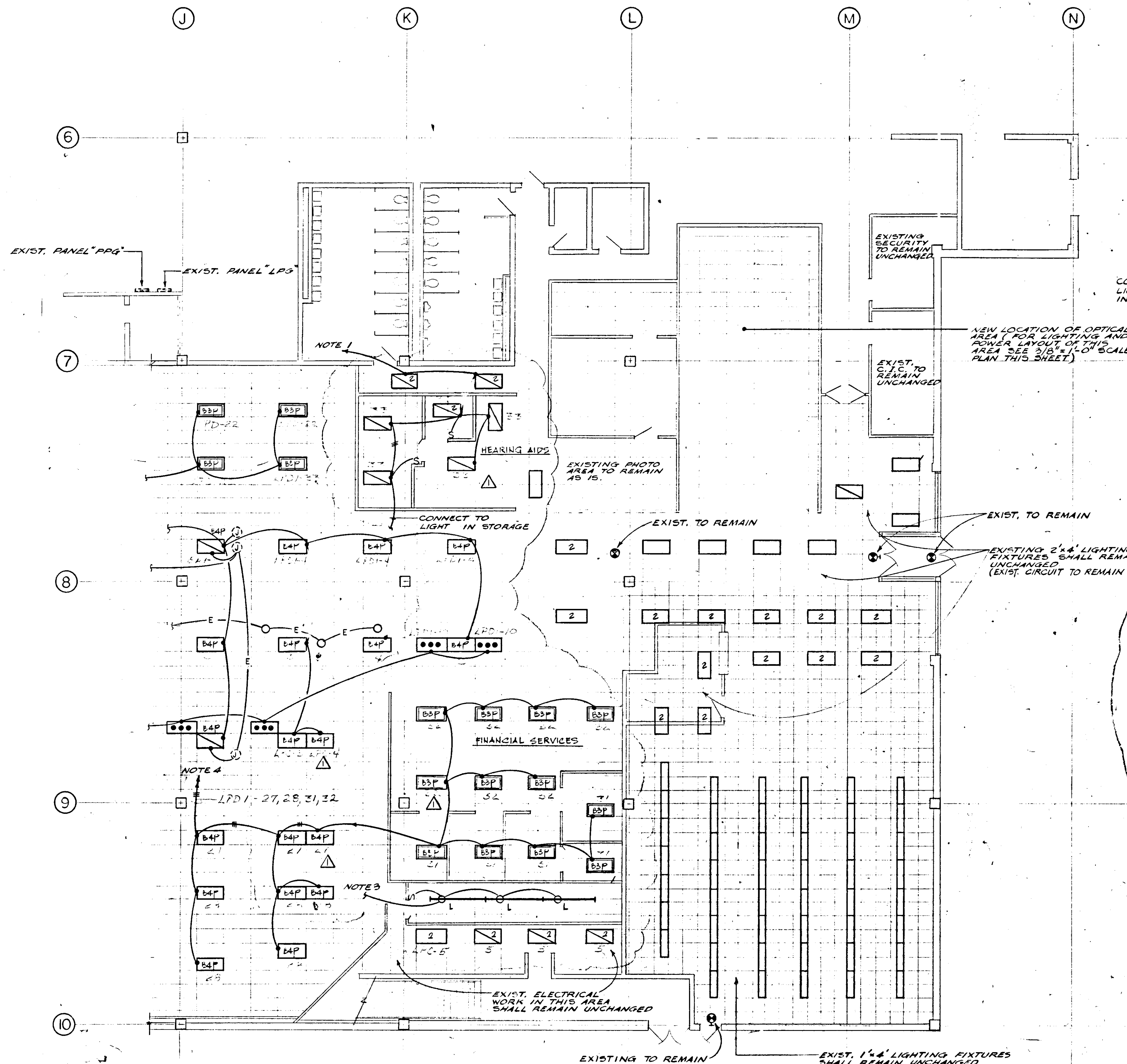
FIRST FLOOR - LIGHTING SCALE: 1/8" = 1'-0"
