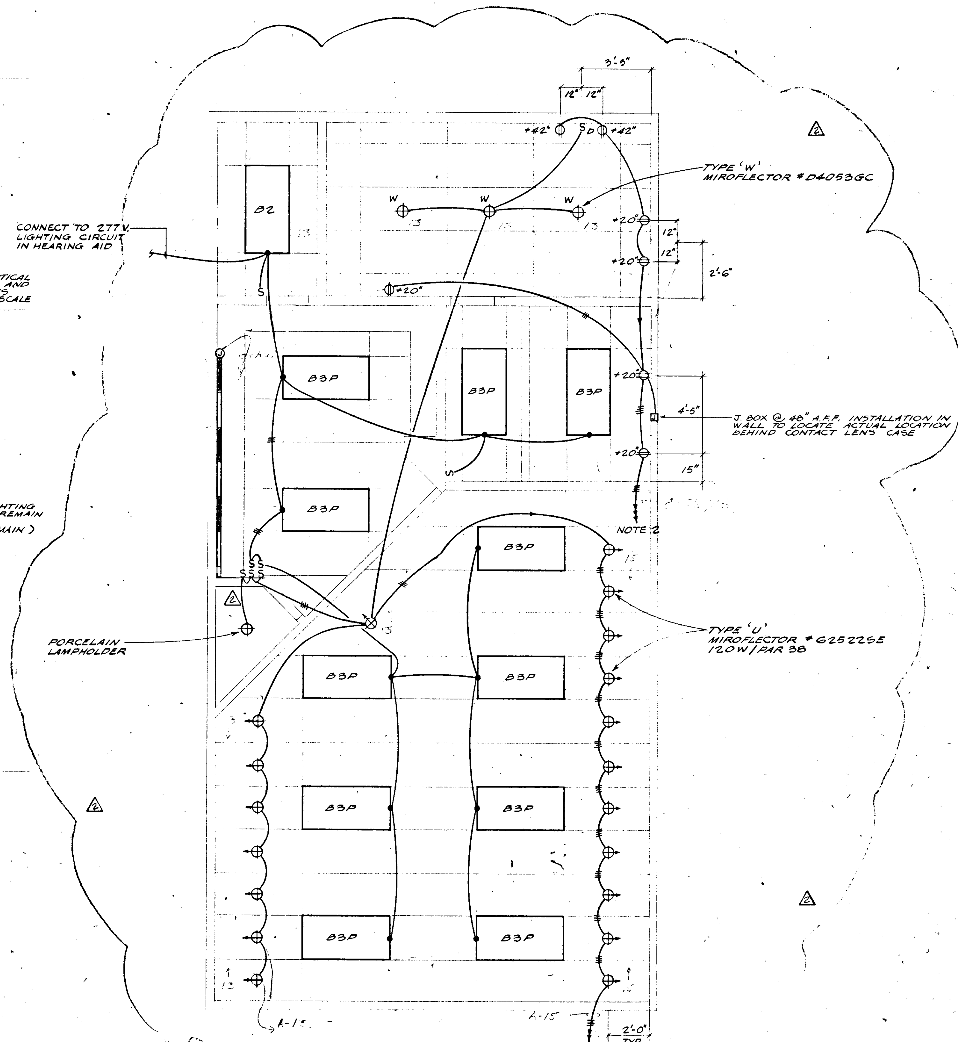
OPTICAL OPTOMETRIST LIGHTING & POWER PLAN SCALE: 3/8" = 1'-0"
