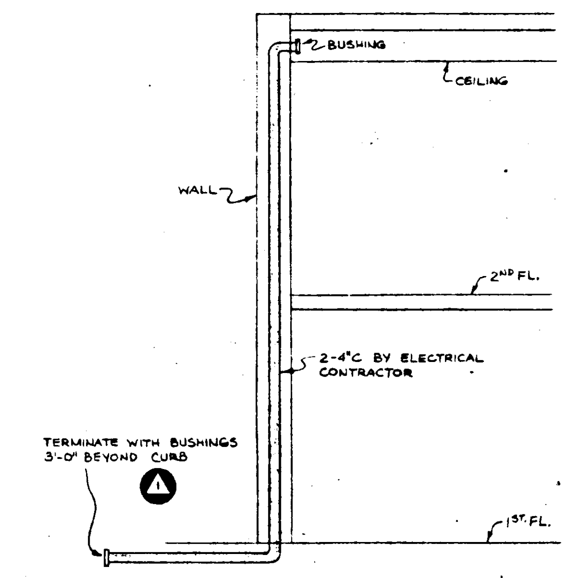
TELEPHONE CONDUITS - DETAIL NO SCALE
