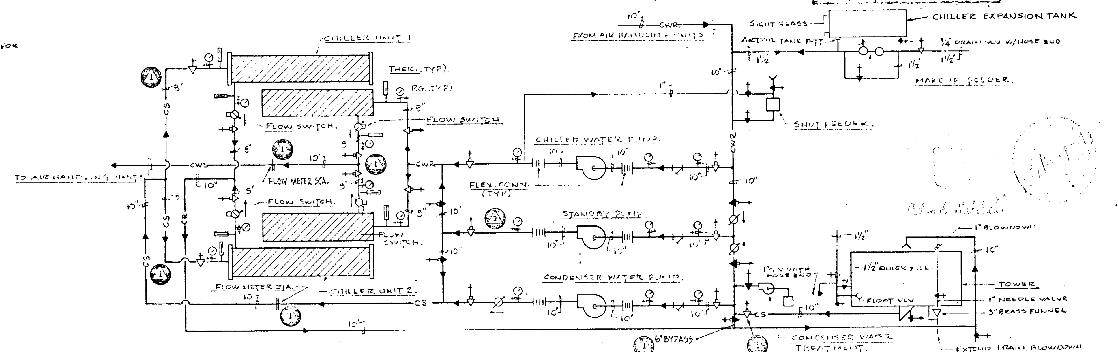
SCHEMATIC CHILLED/CONDENSER WATER SYSTEM
