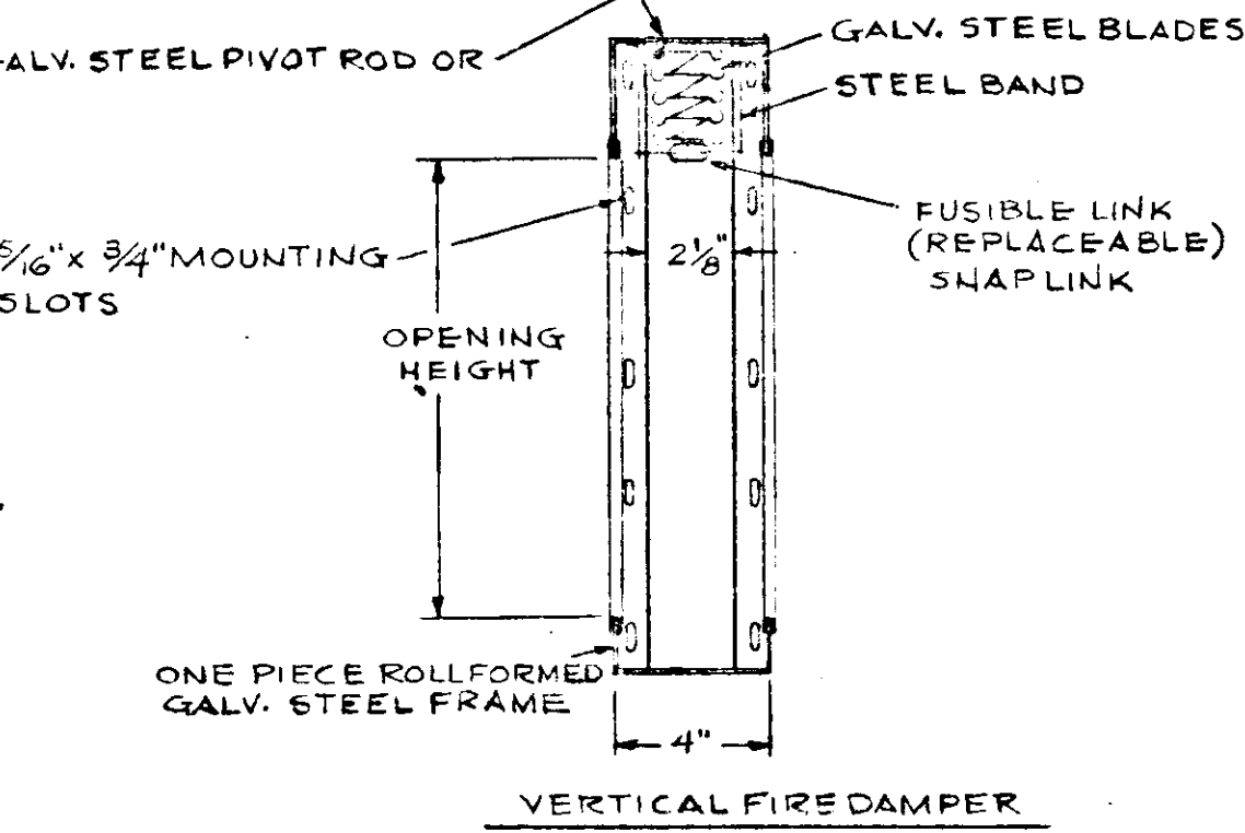
TYPICAL FIRE DAMPER DETAIL AT MASONRY OPENING NO SCALE
