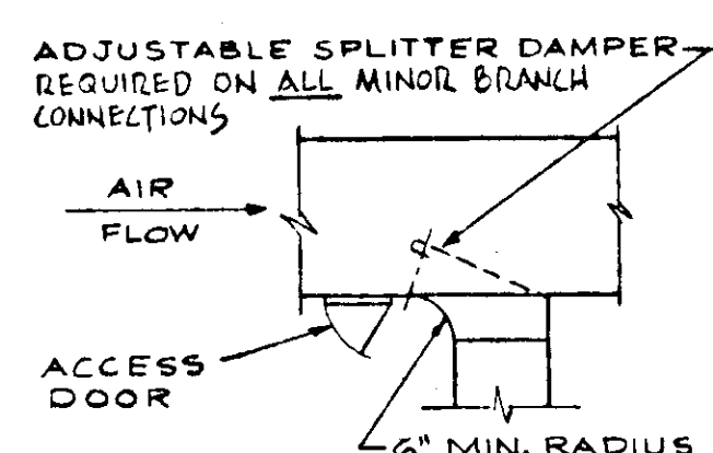
TYP. MINOR BRANCH CONN. DET. NO SCALE
