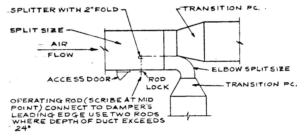
TYPICAL BRANCH CONNECTION DETAIL NO SCALE
