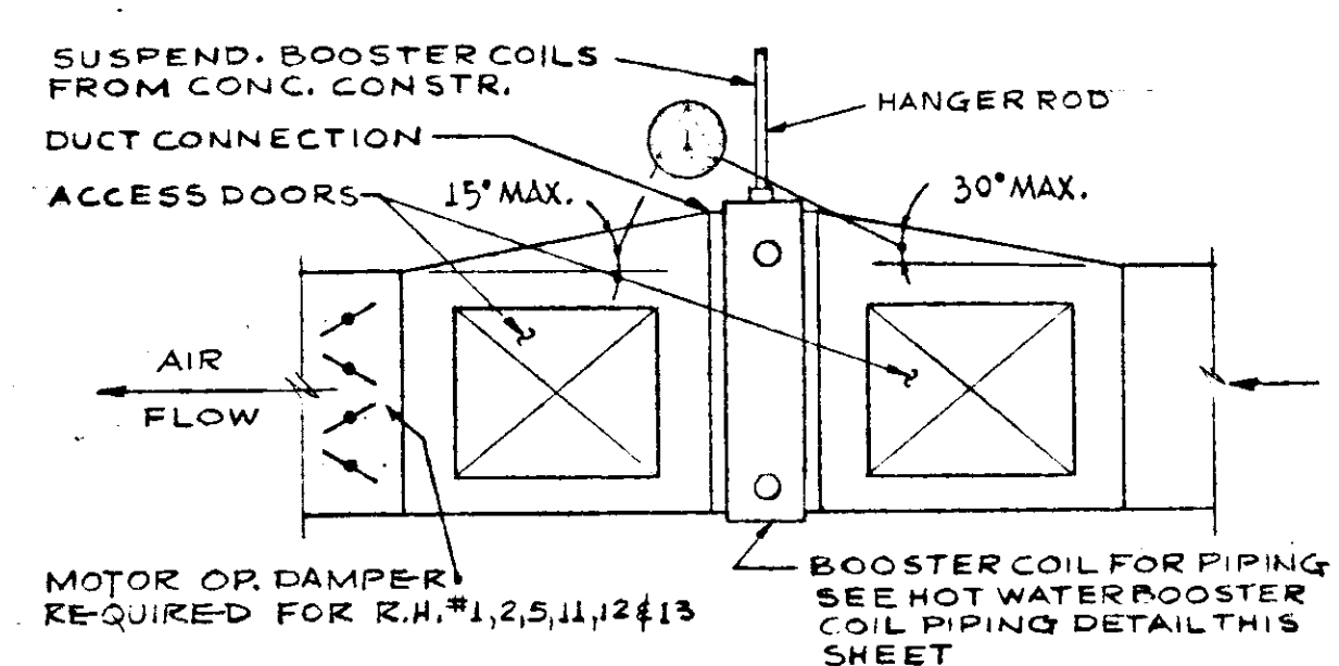
TYPICAL BOOSTER COIL DETAIL NO SCALE
