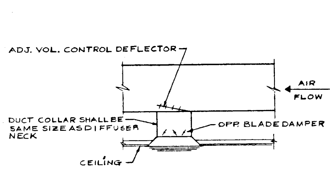
TYPICAL DIFFUSER TAKEOFF DET. NO SCALE
