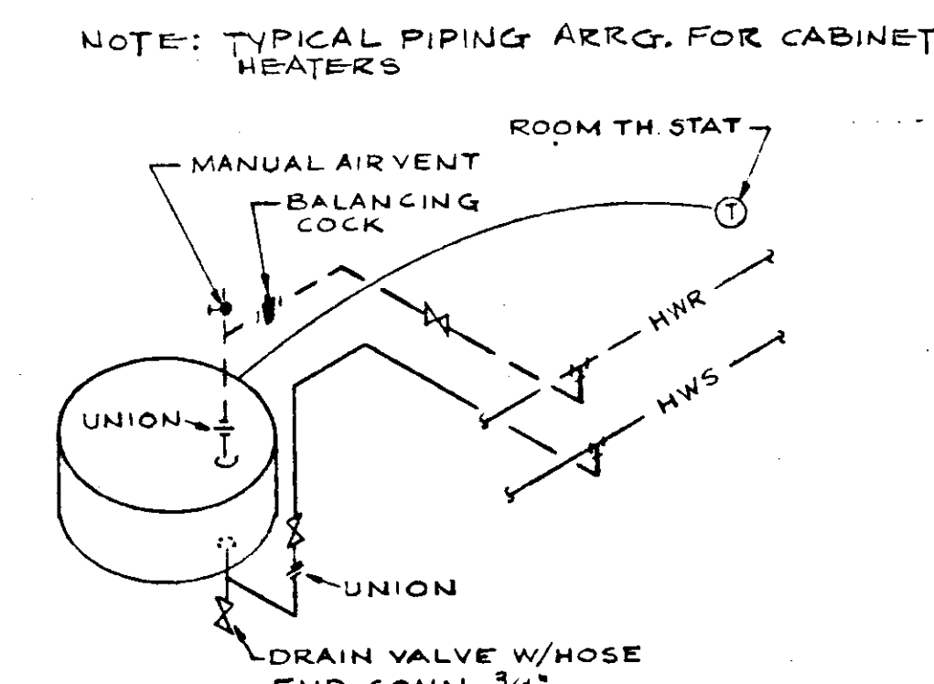
HOT WATER VERT. UNIT HEATER DET. NO SCALE
