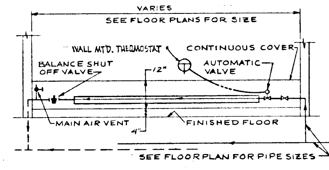
HOT WATER FINNED TUBE RADIATION DETAIL NO SCALE
