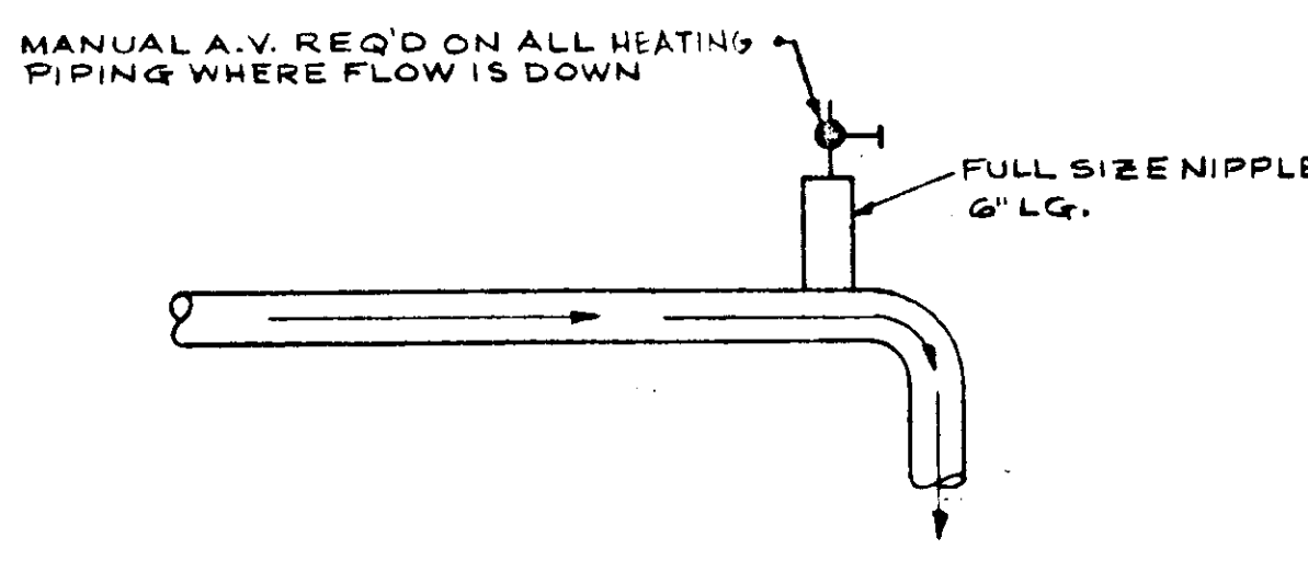
HOT WATER AIR VENT DETAIL NO SCALE
