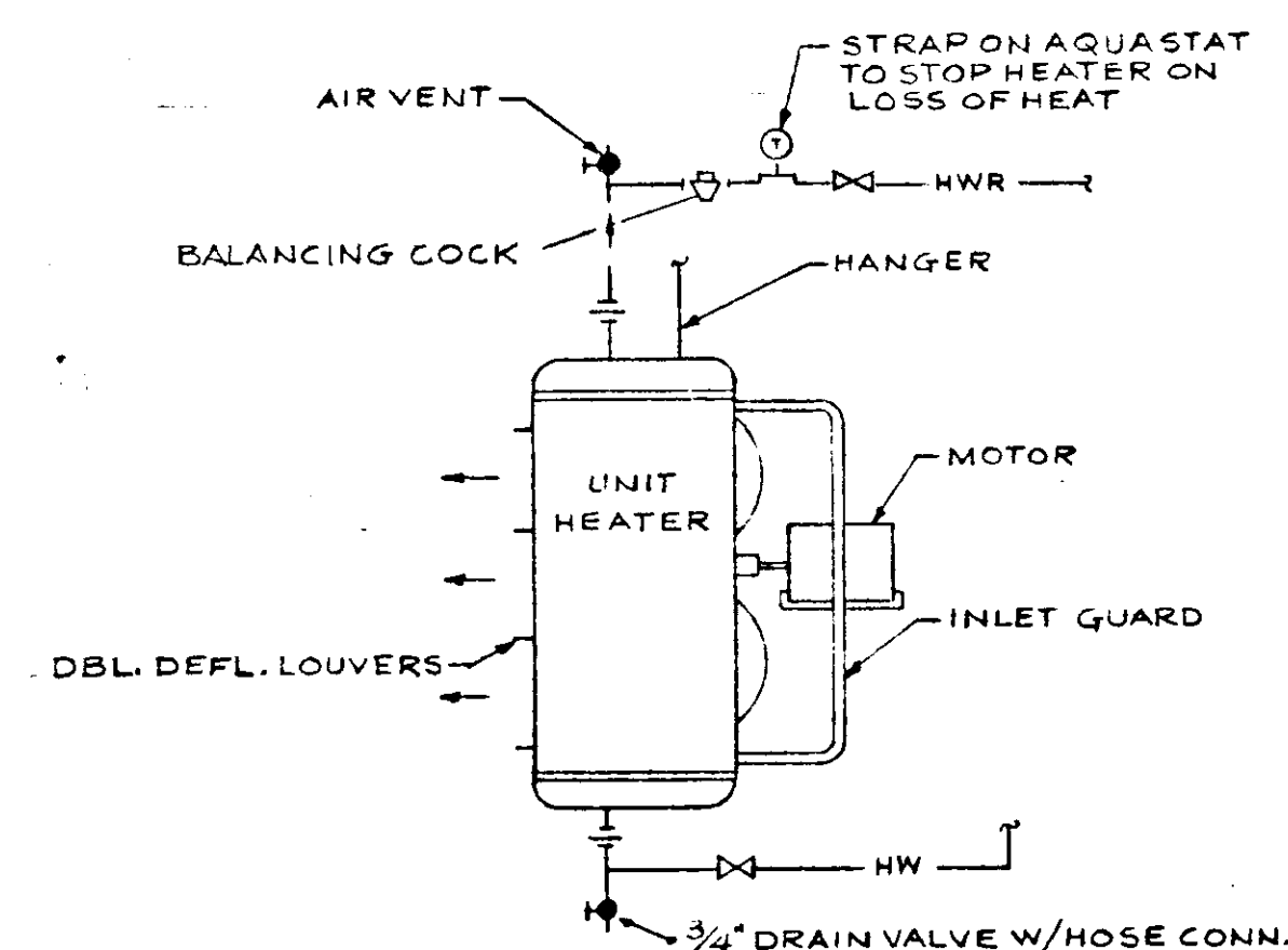
HOT WATER HORIZONTAL UNIT HEATER DET. NO SCALE
