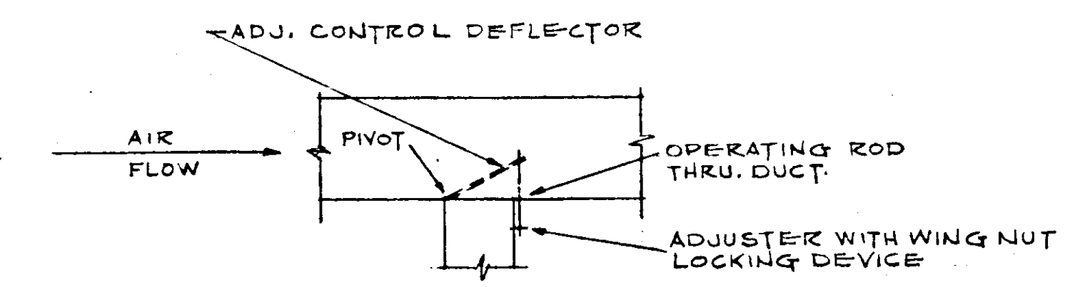
ALTERNATE MINOR BRANCH WHERE SHOWN NO SCALE
