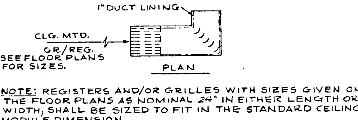
RETURN AIR SOUND TRAP DETAIL NO SCALE
