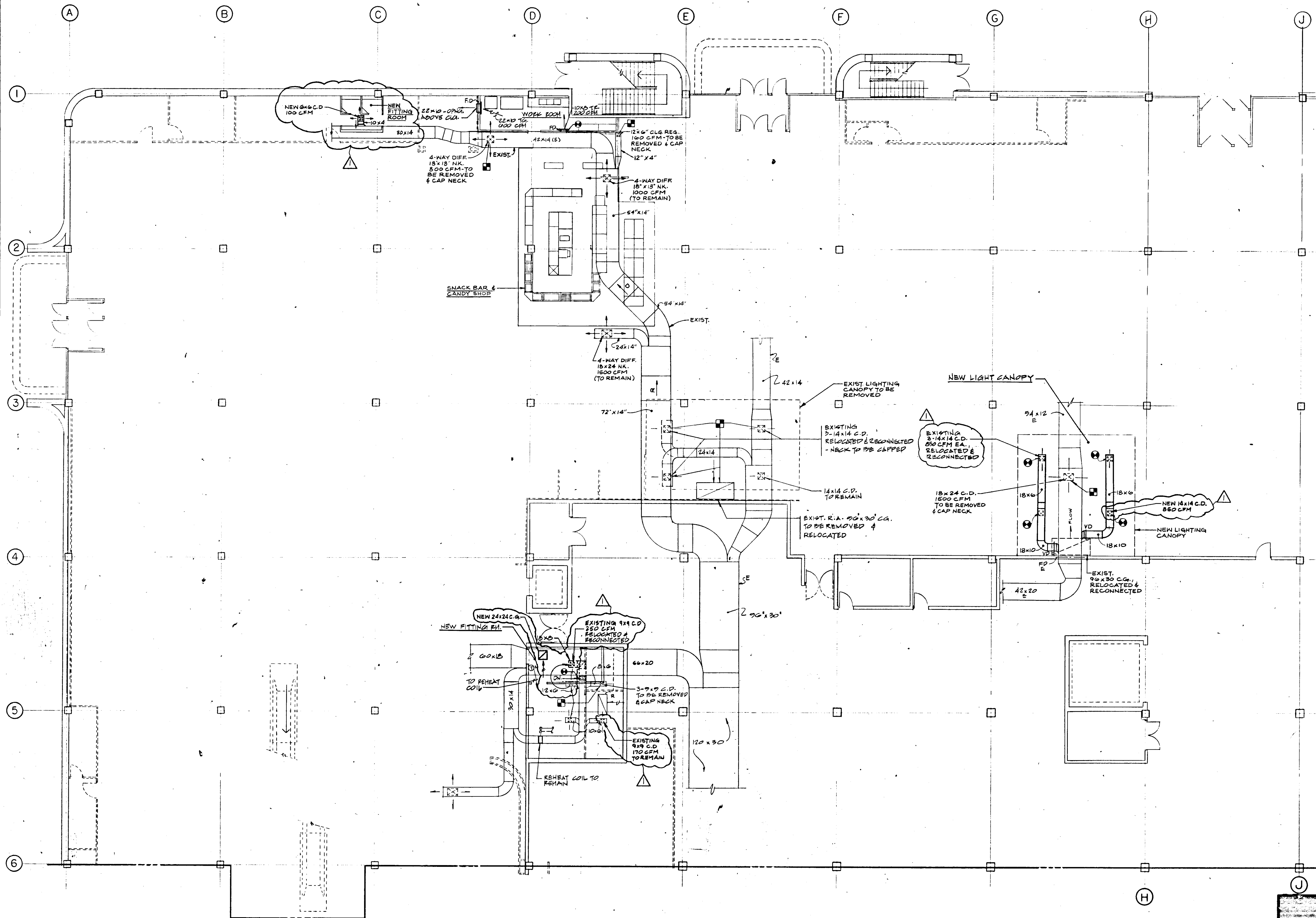
FIRST FLOOR SCALE: 1/8"=1'-0"
