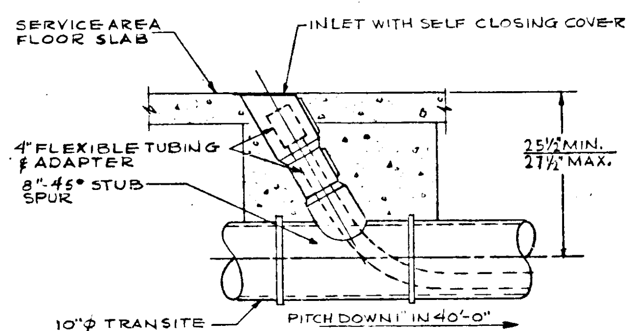
AUTOMOBILE EXHAUST INLET DETAIL NO SCALE
