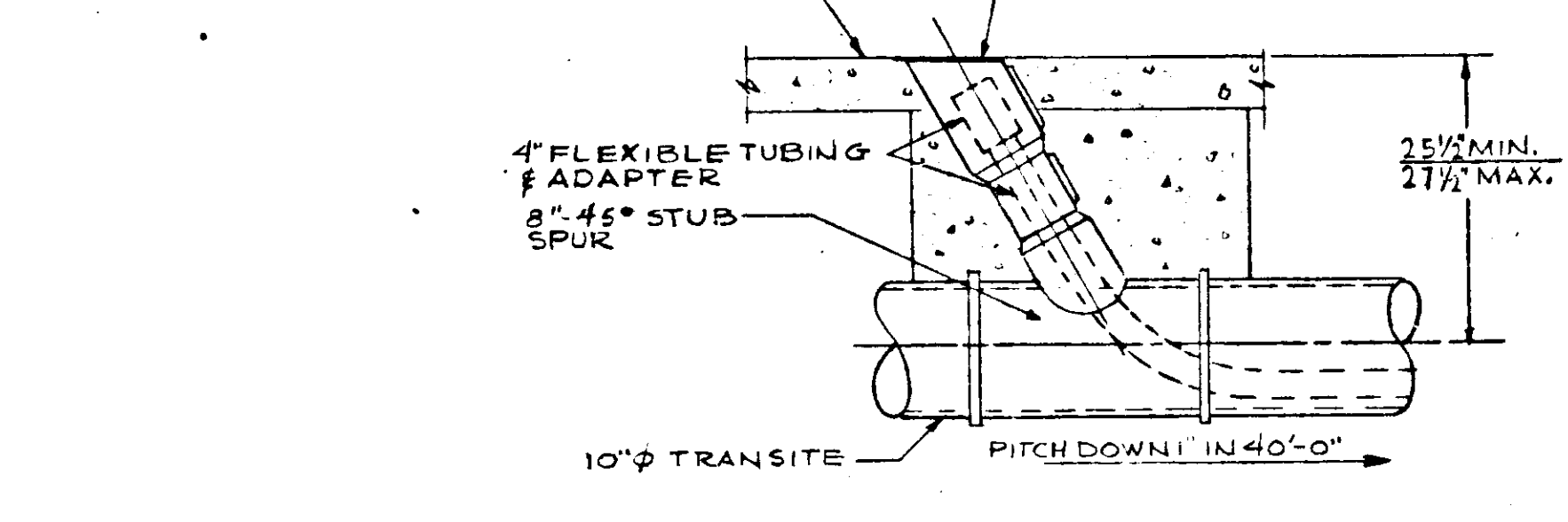
AUTOMOBILE EXHAUST INLET DETAIL NO SCALE
