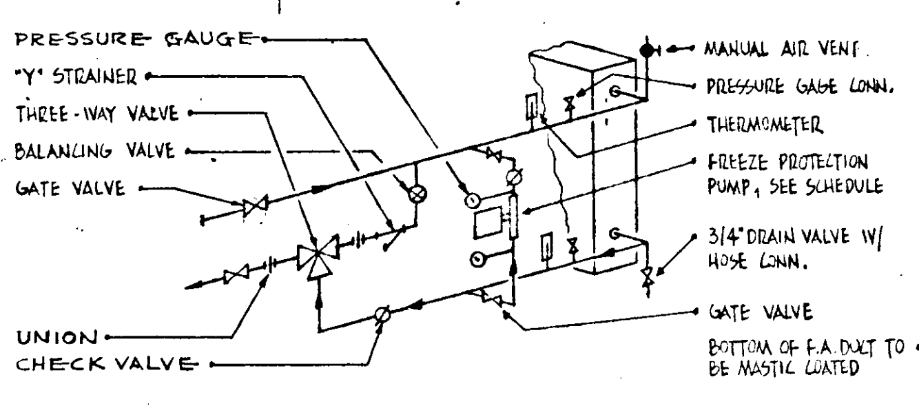
H/V UNITS HOT WATER COIL DETAIL NO SCALE
