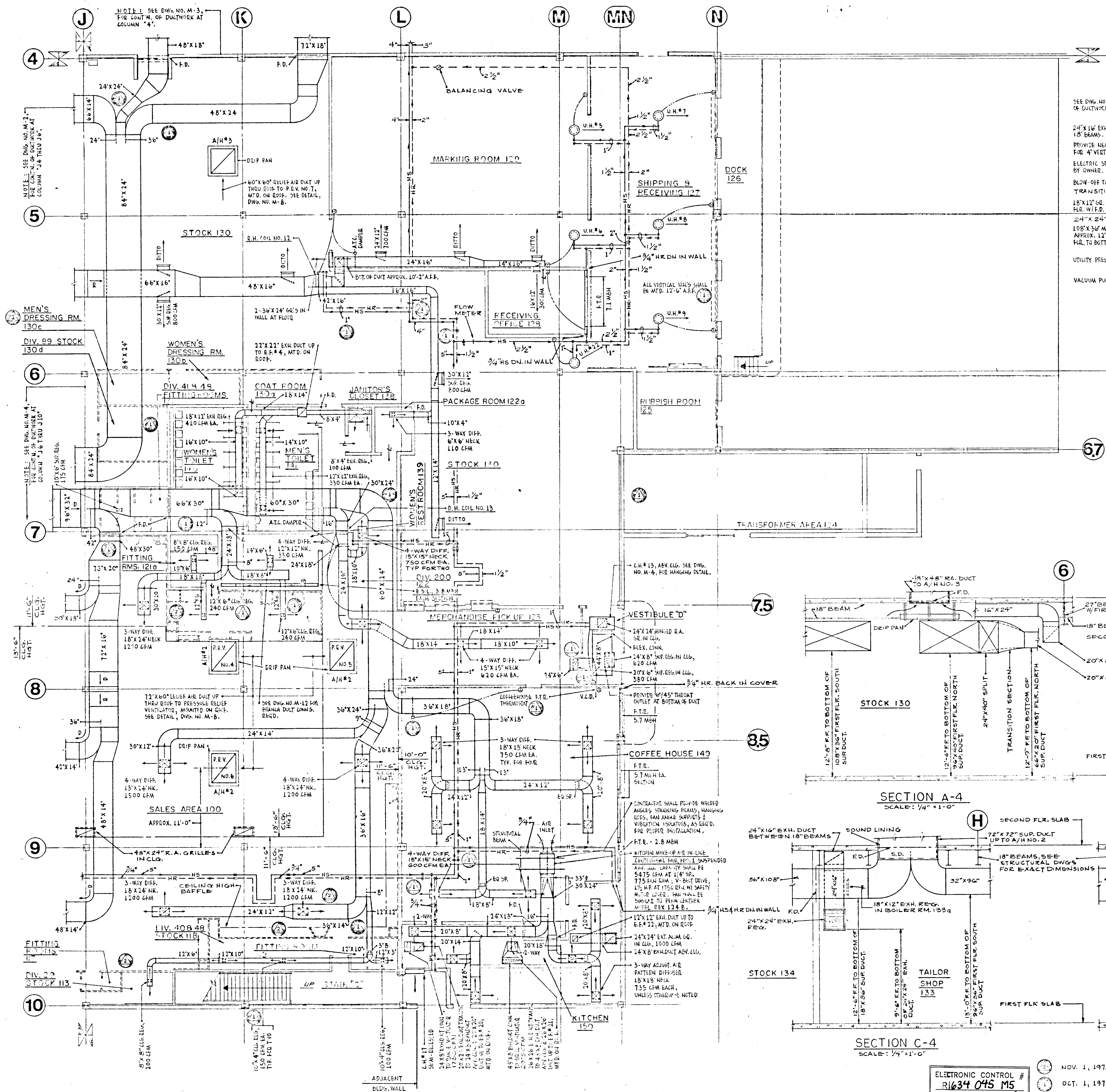
TAILOR SHOP 133 & BOILER ROOM 133A FLOOR PLAN SCALE: 1/4" = 1'-0"
