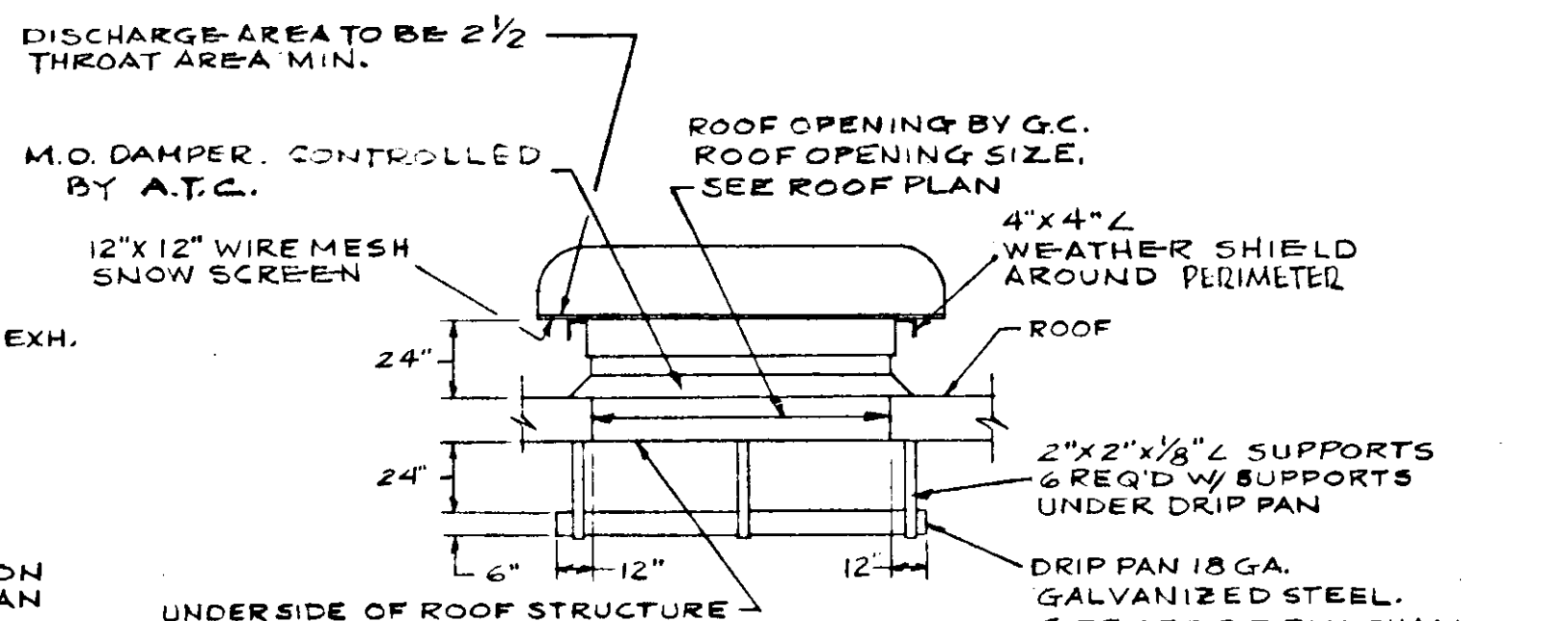
PRESSURE RELIEF VENTILATOR DETAIL
