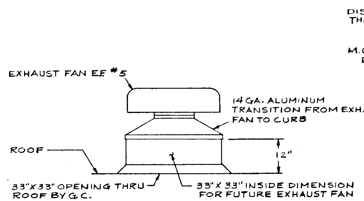
EXHAUST FAN NO. 5 MOUNTING DETAIL NO SCALE
