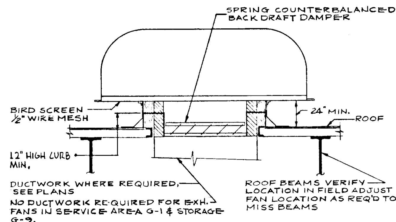
EXHAUST FAN MOUNTING DETAIL NO SCALE
