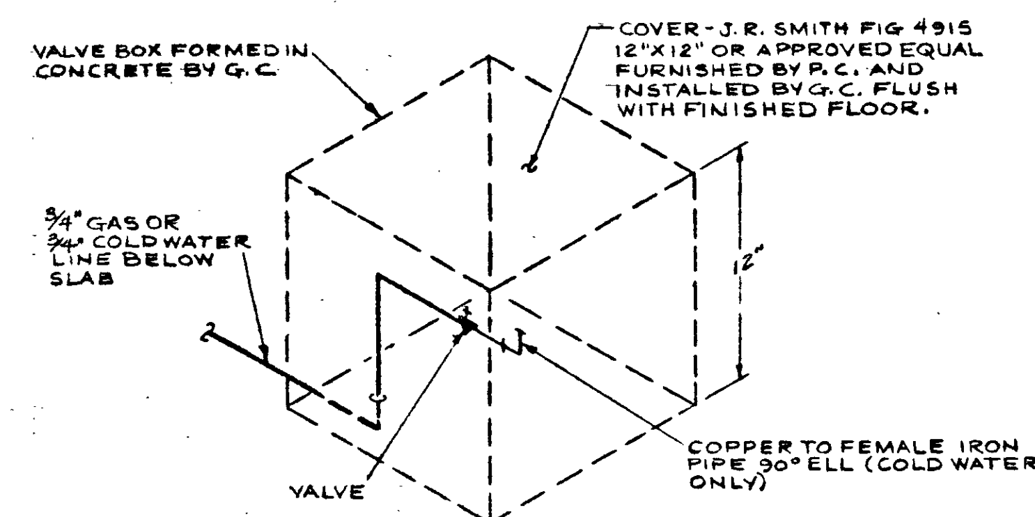
TYPICAL DETAIL - VALVE BOX IN FLOOR FOR GAS & WATER OUTLETS IN DISPLAY AREA (SEE PLAN FOR LOCATIONS) NO SCALE
