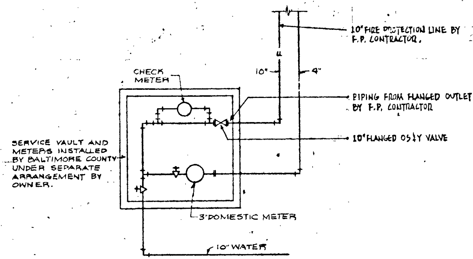
METER VAULT DETAIL NO SCALE
