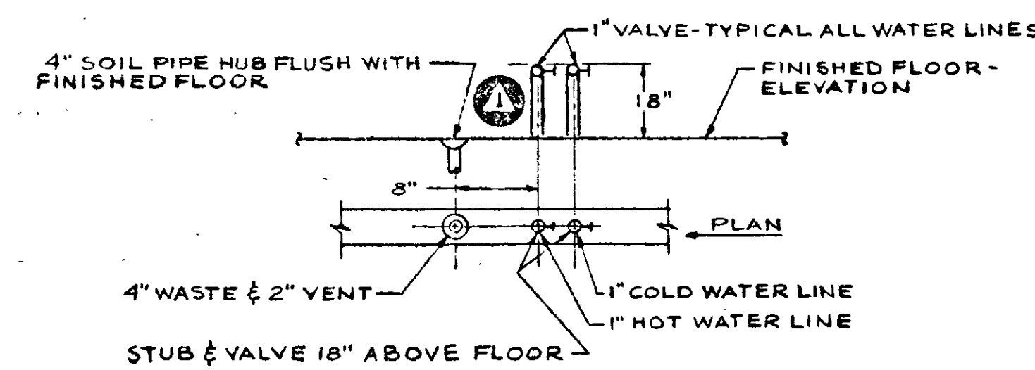
TYPICAL DETAIL - LAUNDRY DISPLAY PLUMBING NO SCALE
