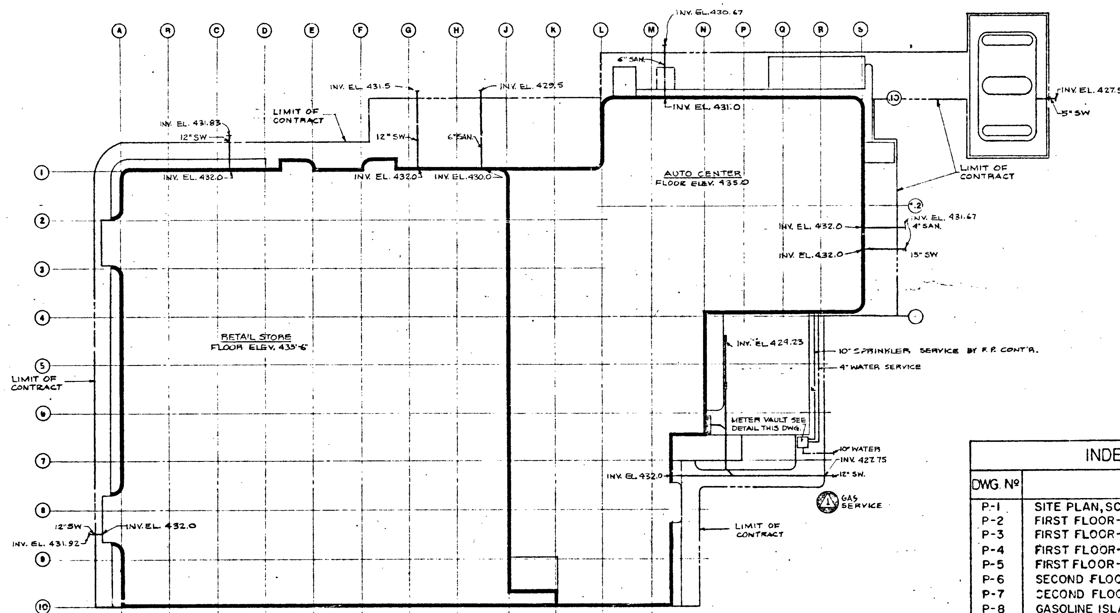
SITE PLAN SCALE: 1/4" = 1'-0"
