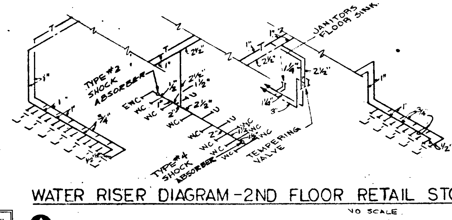
WATER RISER DIAGRAM-AUTO CENTER-TOILET RM. NO SCALE
