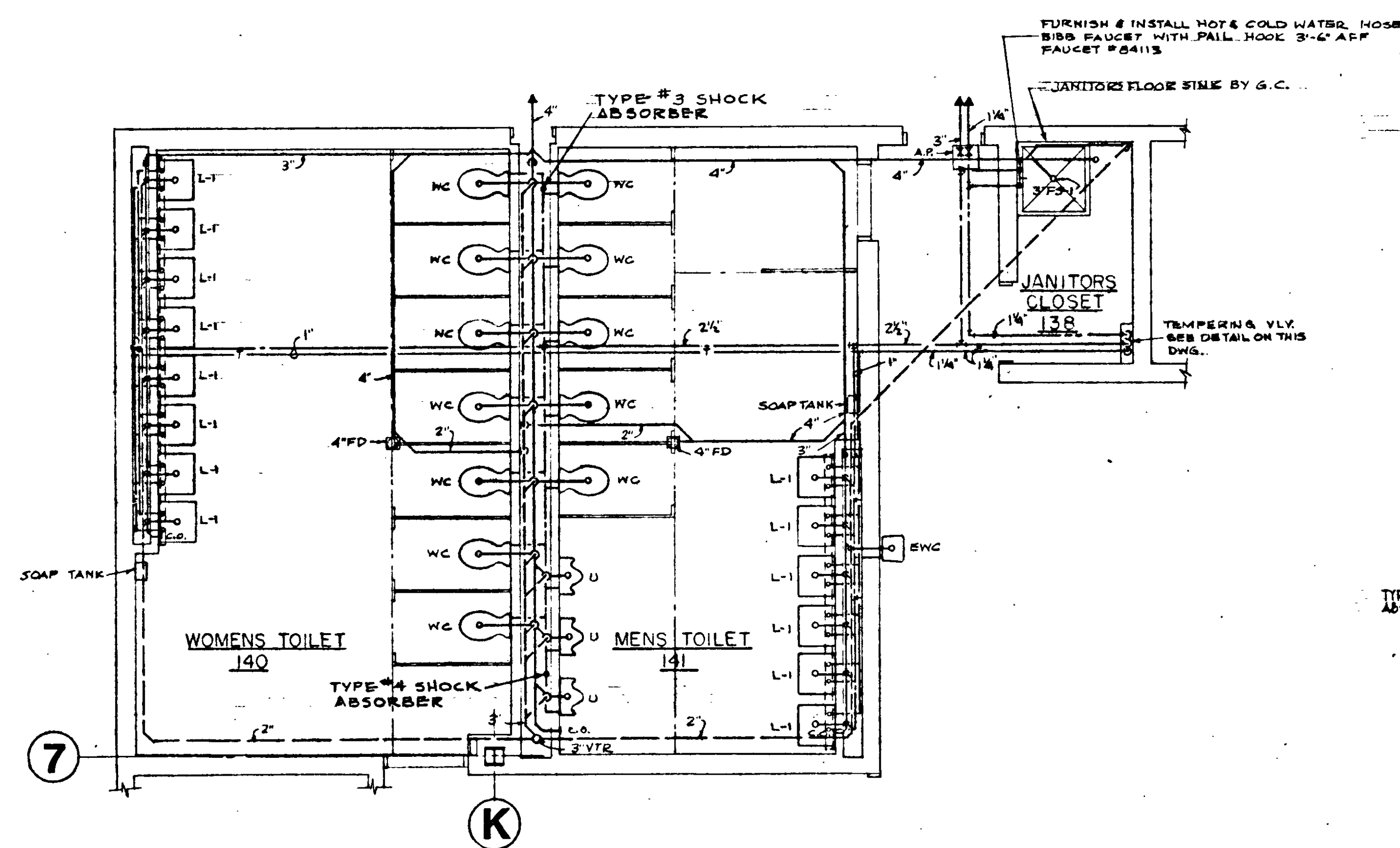
TOILET ROOM PLAN FIRST FLOOR RETAIL STORE SCALE: 1/4"=1'-0"
