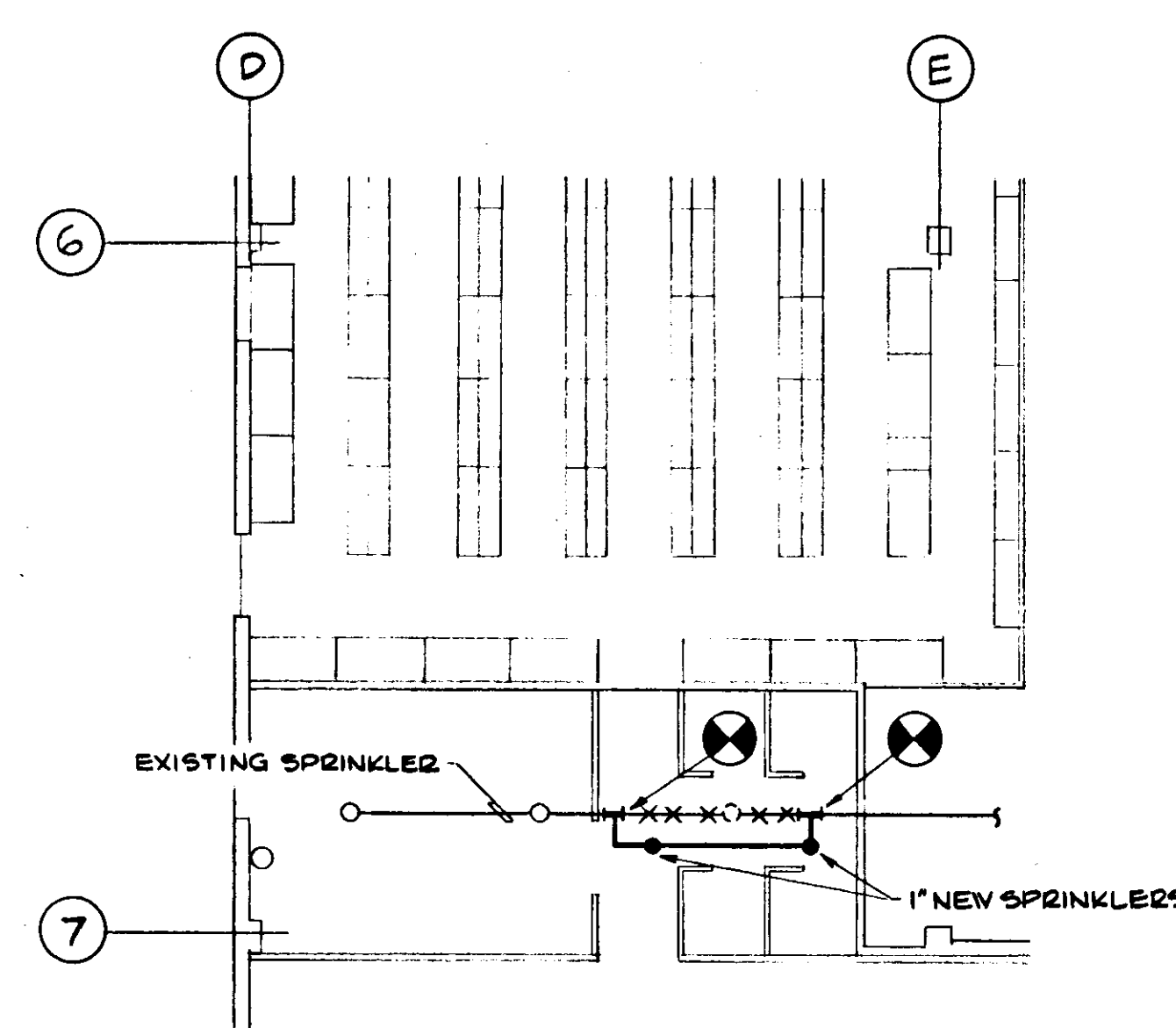
PARTIAL PLAN# 3 - FIRST FLOOR SCALE: 1/8" = 1'-0"
