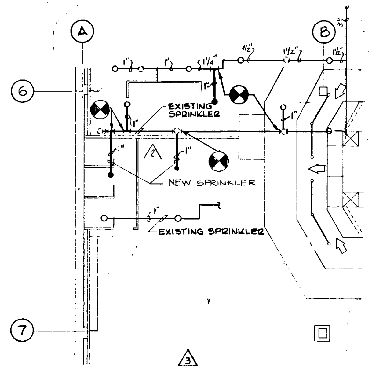
PARTIAL PLAN# 2 - FIRST FLOOR SCALE: 1/8" = 1'-0"
