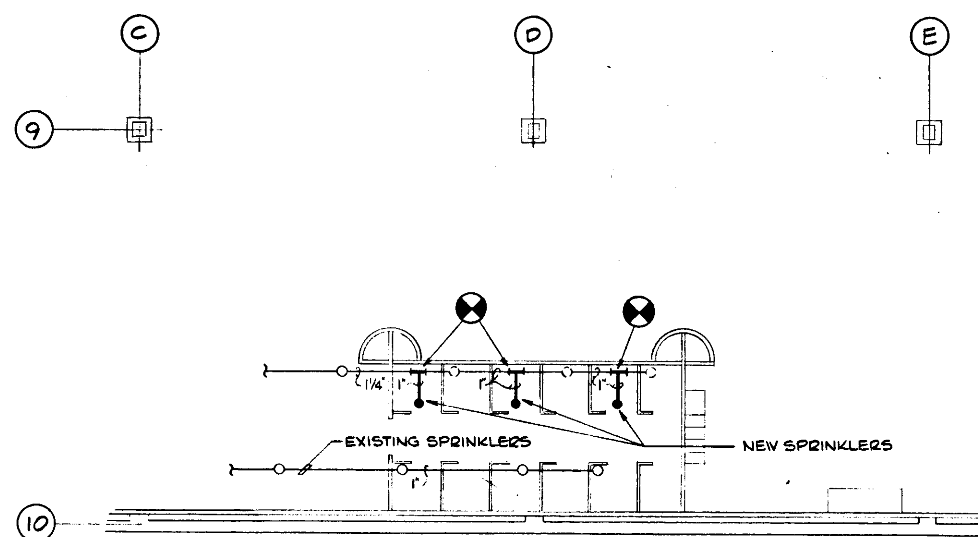
PARTIAL PLAN# 1 - FIRST FLOOR SCALE: 1/8" = 1'-0"
