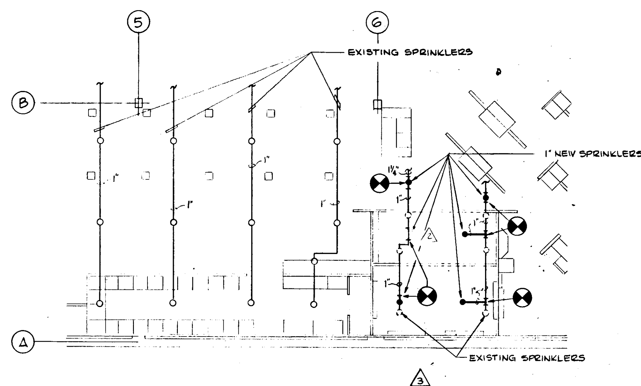
PARTIAL PLAN# 6 - SECOND FLOOR SCALE: 1/8" = 1'-0"
