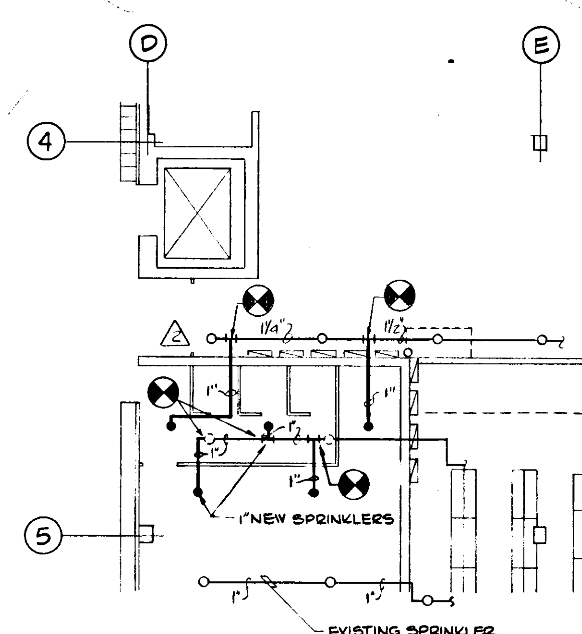
PARTIAL PLAN# 4 - FIRST FLOOR SCALE: 1/8" = 1'-0"
