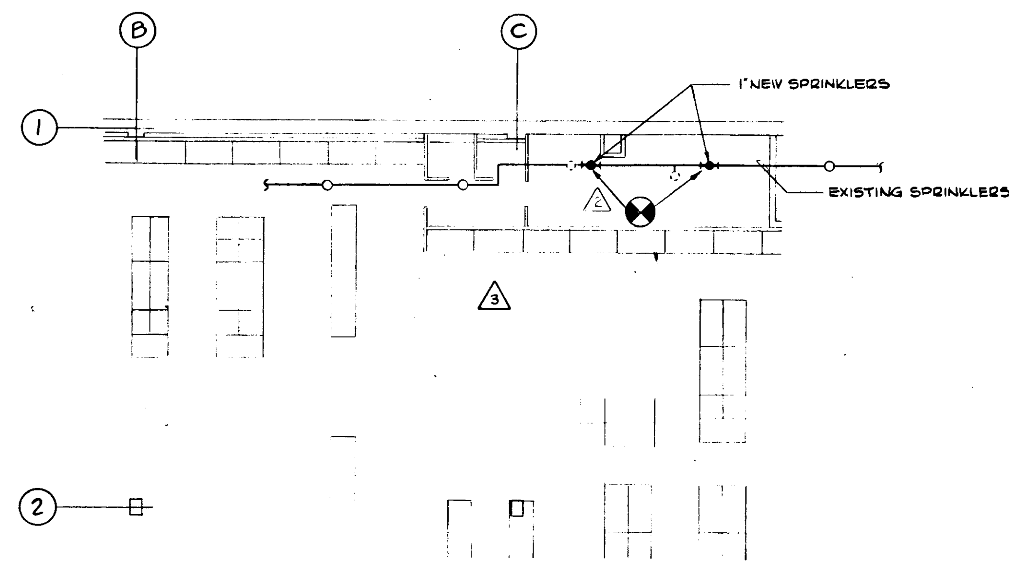
PARTIAL PLAN# 5 - FIRST FLOOR SCALE: 1/8" = 1'-0"
