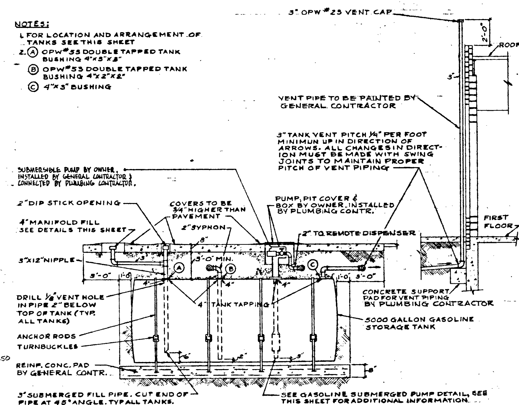
GASOLINE STORAGE TANK DETAIL
