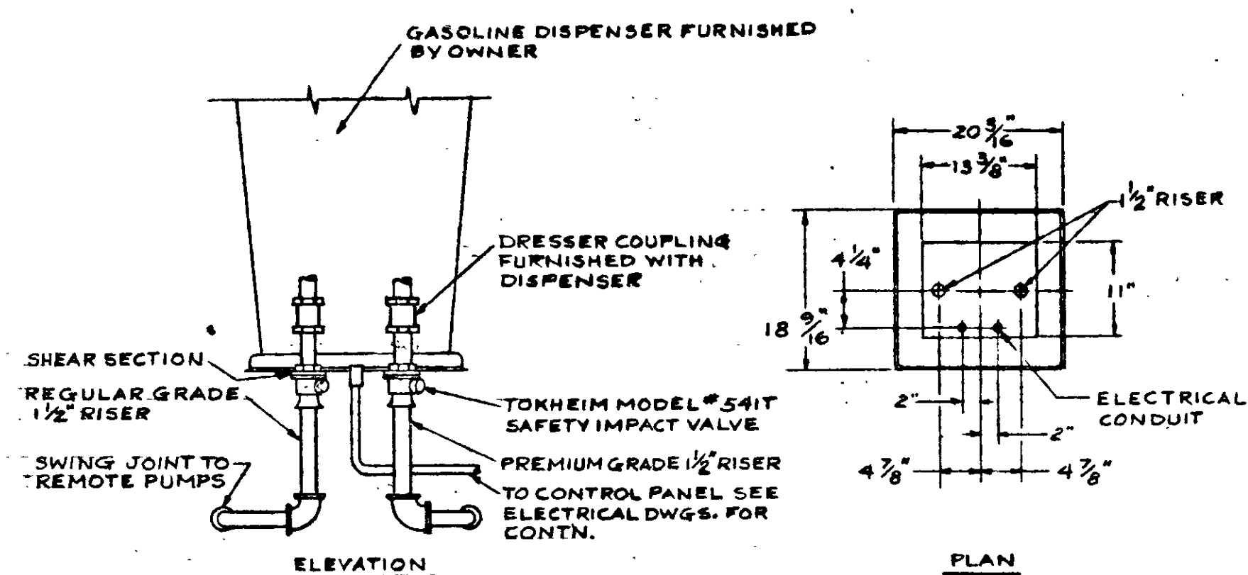
GASOLINE DISPENSER DETAIL
