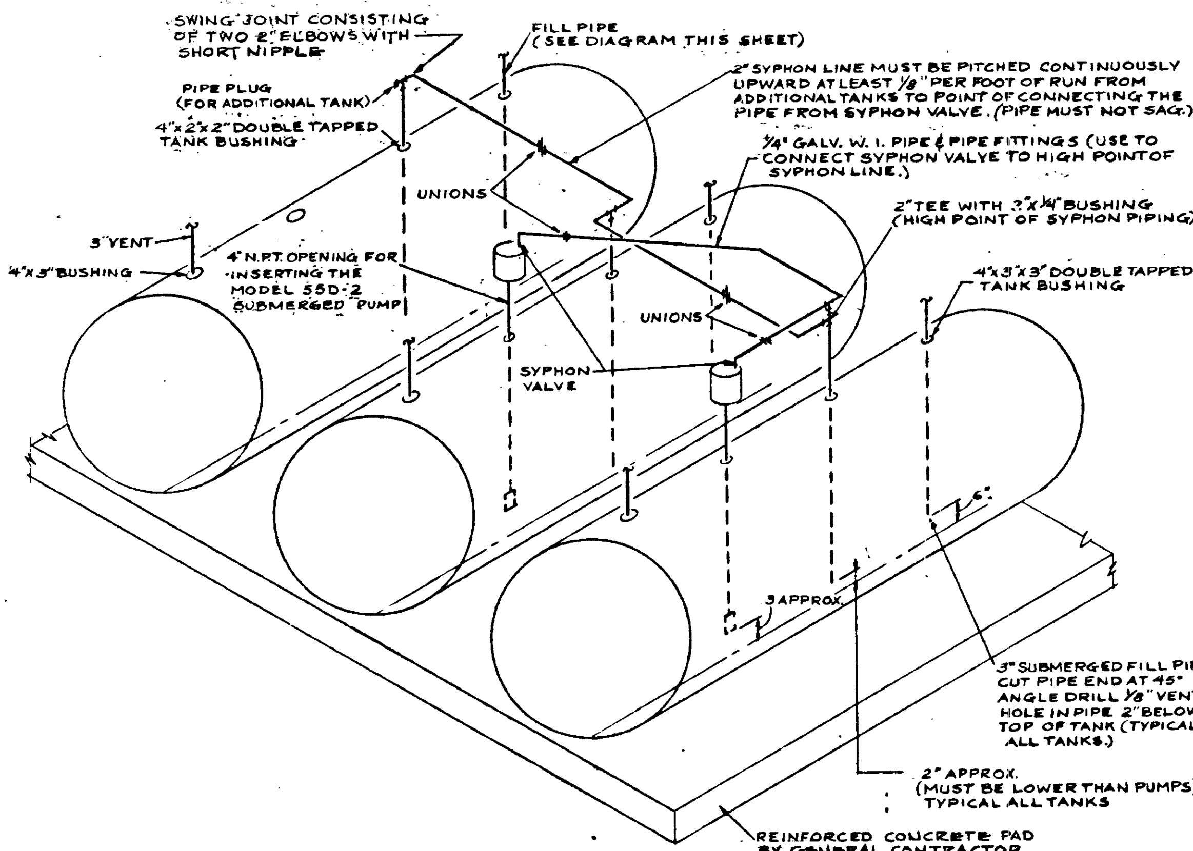
REGULAR GRADE GASOLINE PIPING DIAGRAM
