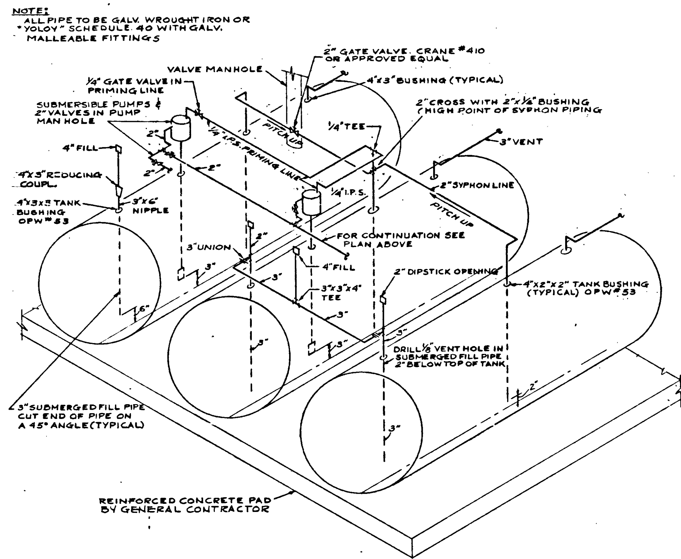
PREMIUM FUTURE GRADE GASOLINE PIPING DIAGRAM
