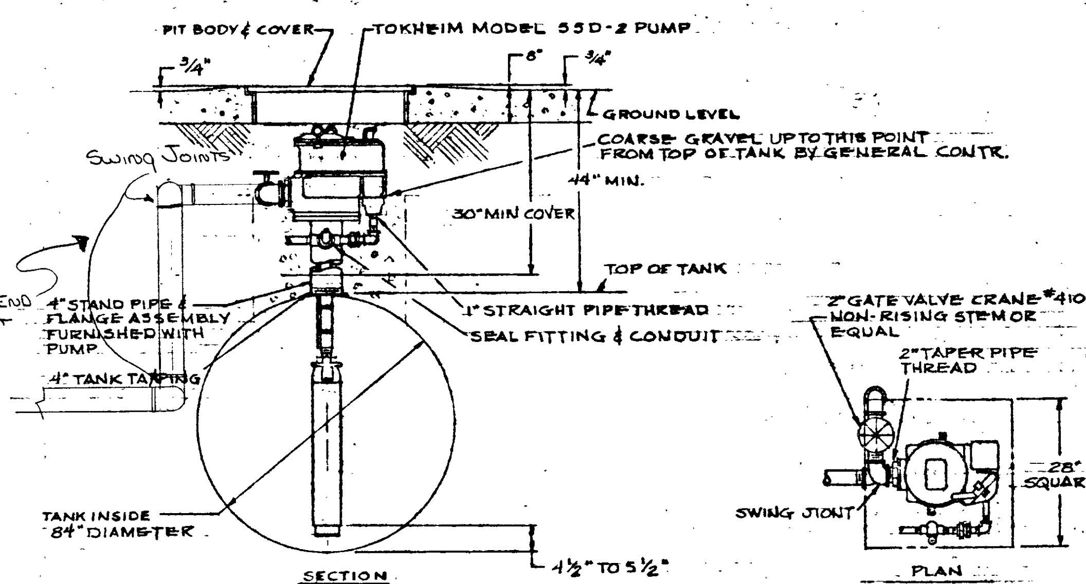
GASOLINE STORAGE TANK DETAIL
