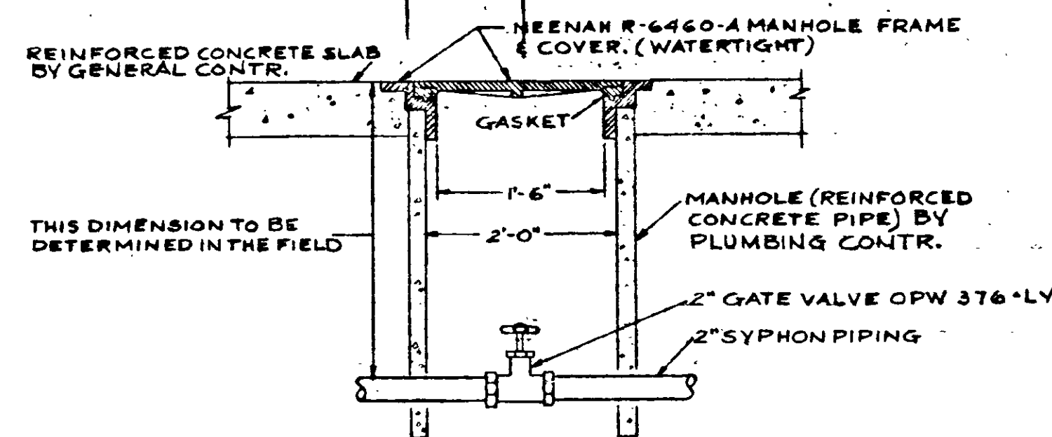
GASOLINE VALVE MANHOLE DETAIL
