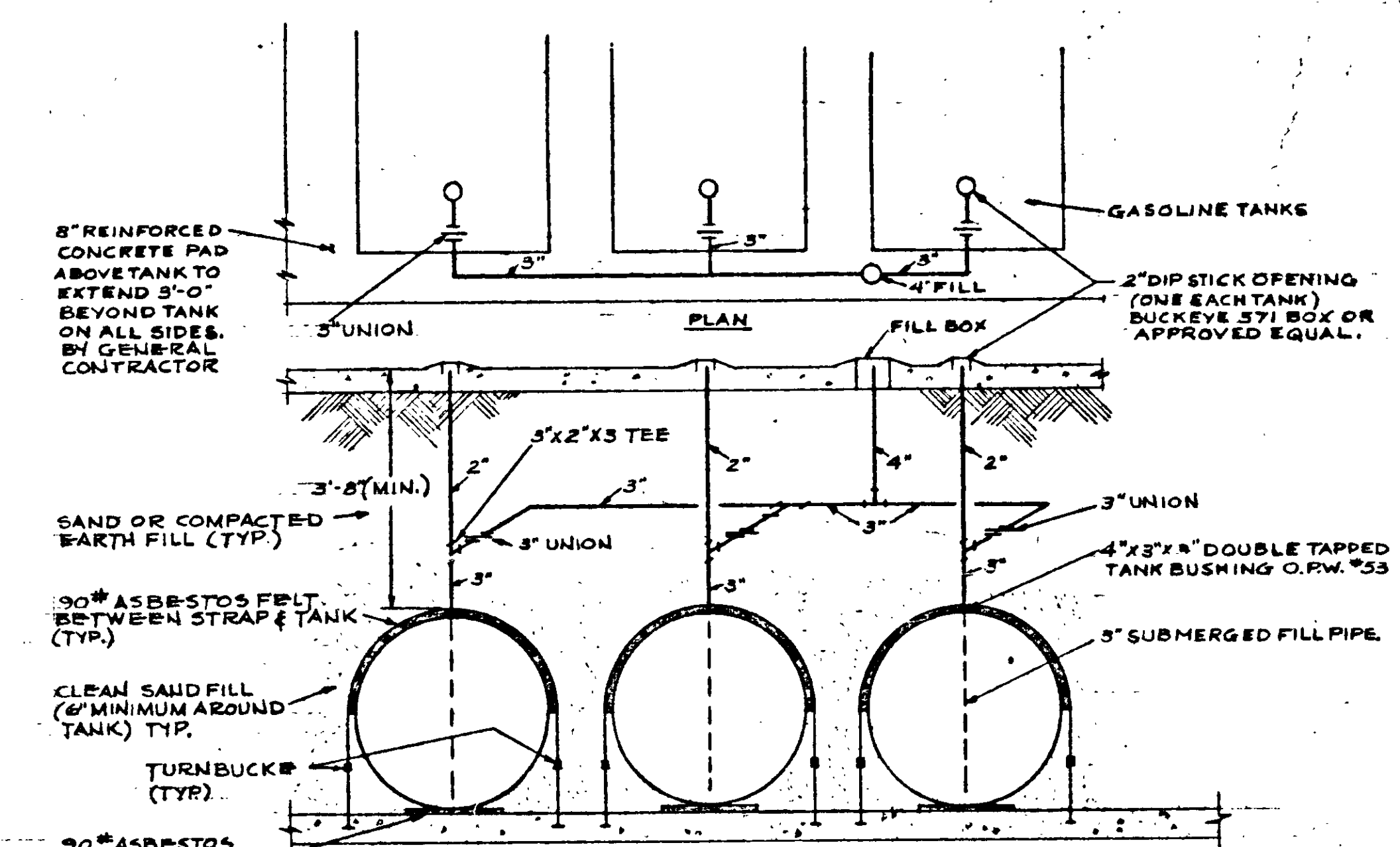
REGULAR GRADE MANIFOLDED GASOLINE FILL DETAIL
