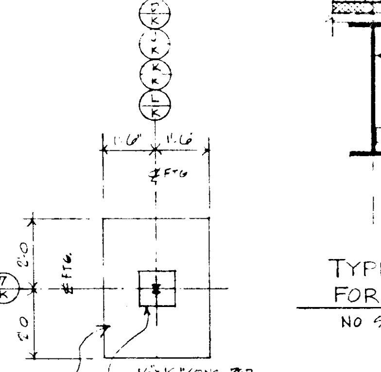
FOOTING DETAIL G SCALE: 3/8" = 1'-0"
