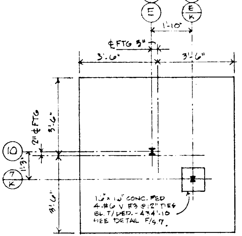
FOOTING DETAIL B SCALE: 3/8" = 1'-0"
