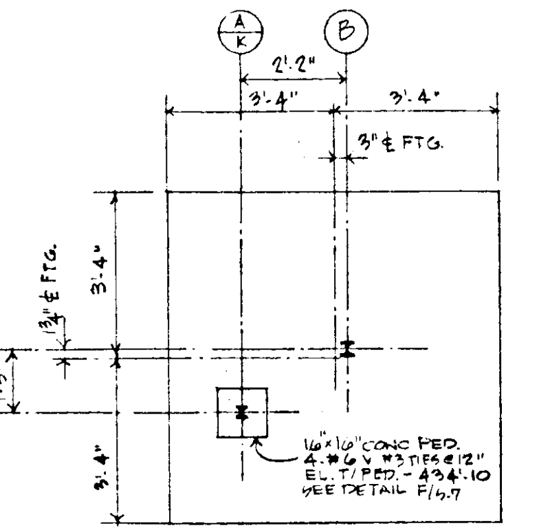
FOOTING DETAIL A SCALE: 3/8" = 1'-0"
