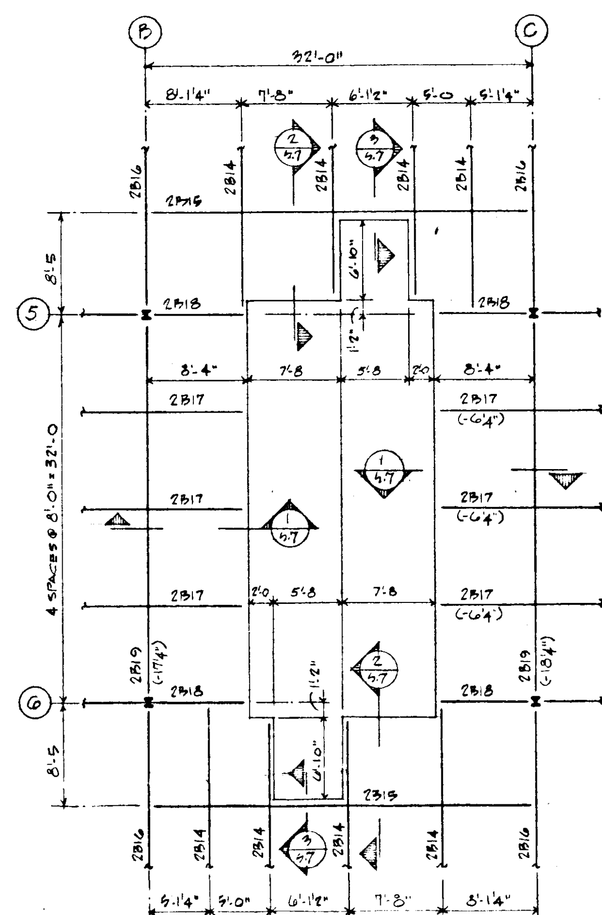
ENLARGED PLAN - ESCALATOR FRAMING SCALE: 1/8" = 1'-0"
