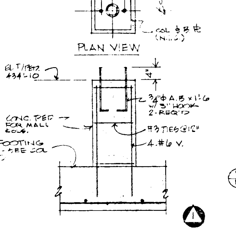
FOOTING DETAIL F SCALE: 3/8" = 1'-0"
