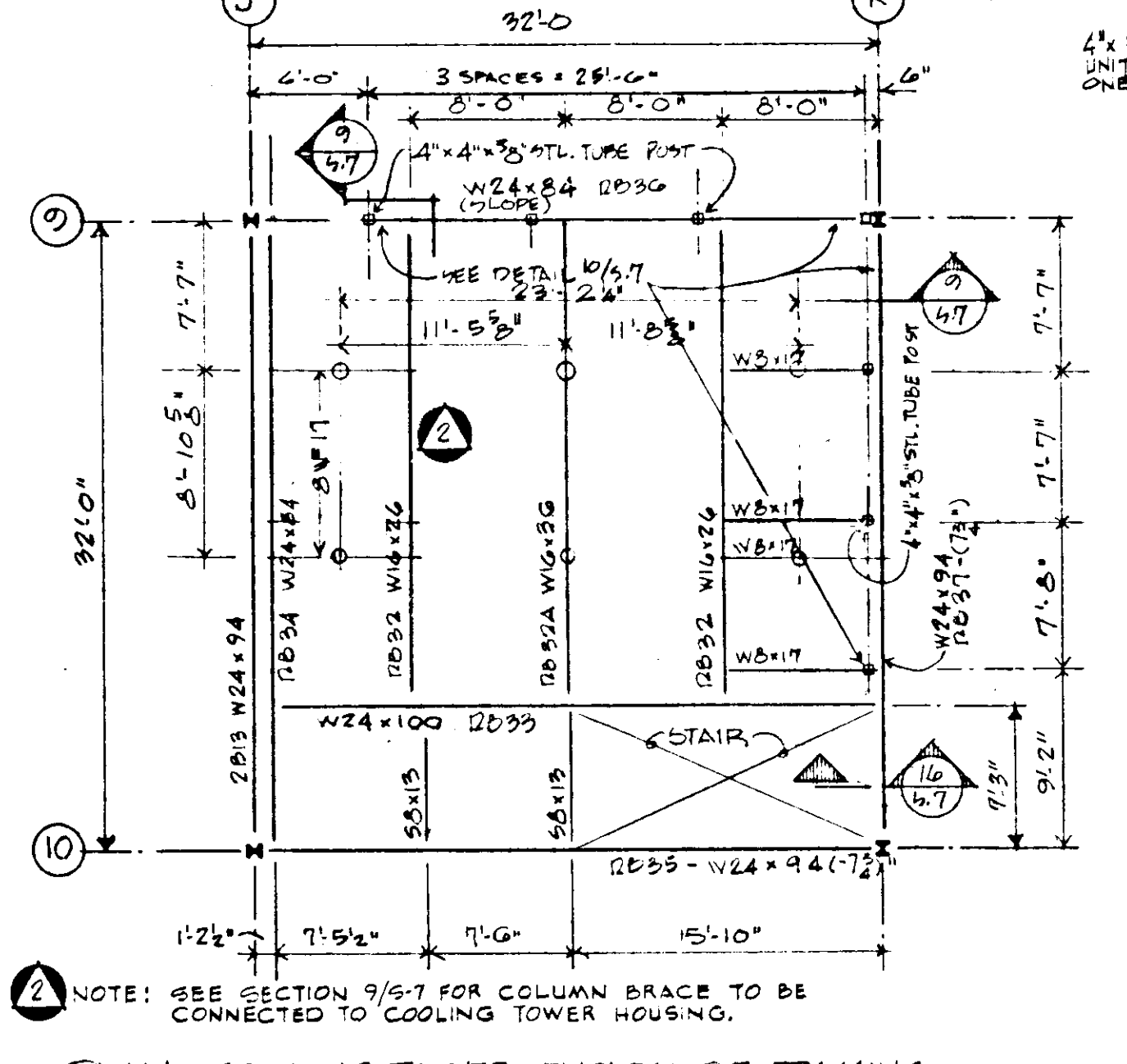
PLAN - COOLING TOWER ENCLOSURE FRAMING SCALE: 1/8" = 1'-0"
