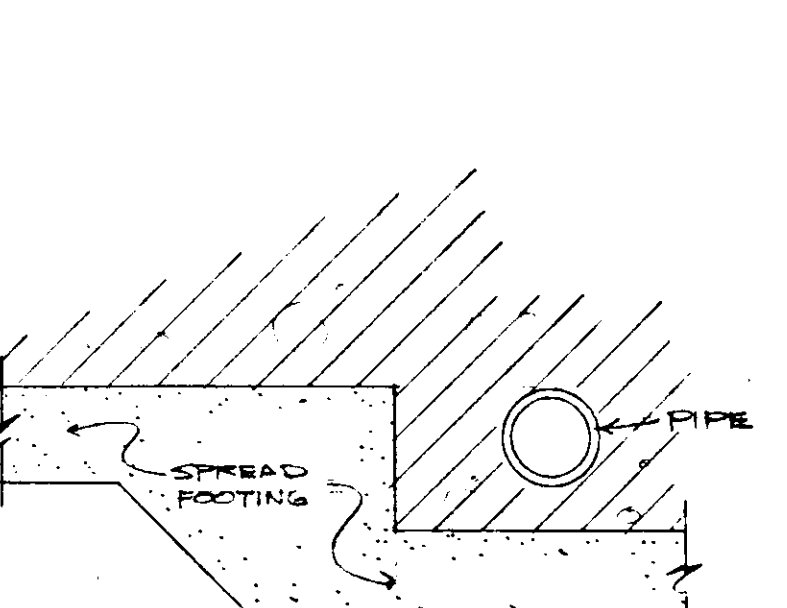
DETAIL - PIPES UNDER GROUND NO SCALE THROUGH WALLS
