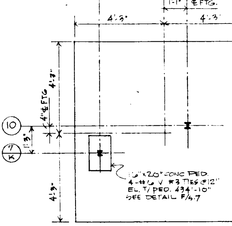
FOOTING DETAIL C SCALE: 3/8" = 1'-0"
